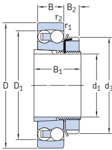
Open bearing
