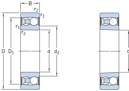
Cylindrical bore
